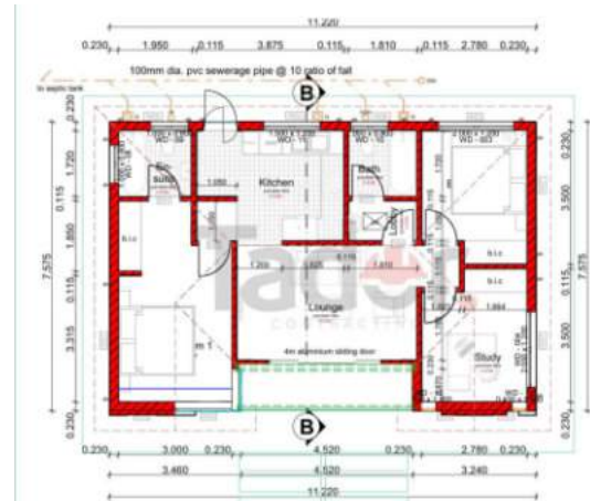
OPTION 01 FLOOR LAYOUT (80sqm)
