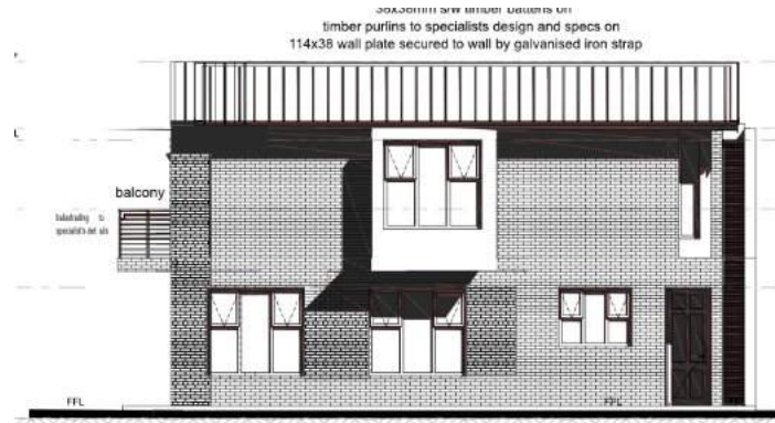
Side Elevation 2
